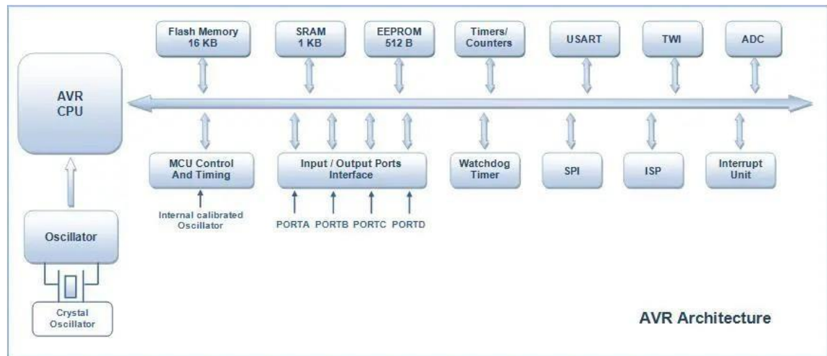
Fig. 5: Block Diagram Explaining AVR Architecture
